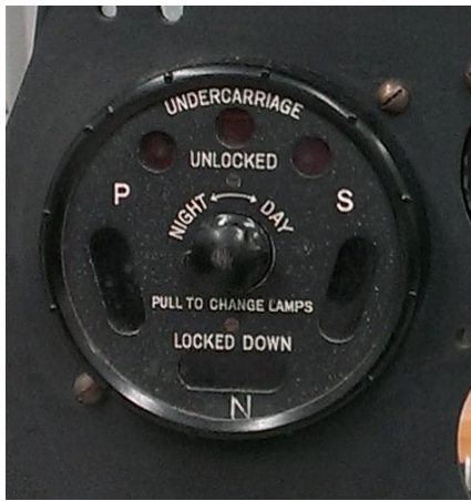
UNDERCARRIAGE POSITION INDICATOR 5C/1009 (NOSE GEAR TYPE)
