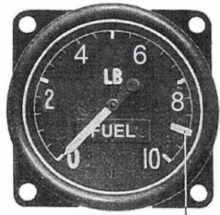
6A/1597 6A/601 Pressure Gauge Mk VIIG Fuel
