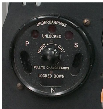
UNDERCARRIAGE POSITION INDICATOR 5C/1009 (NOSE GEAR TYPE)
