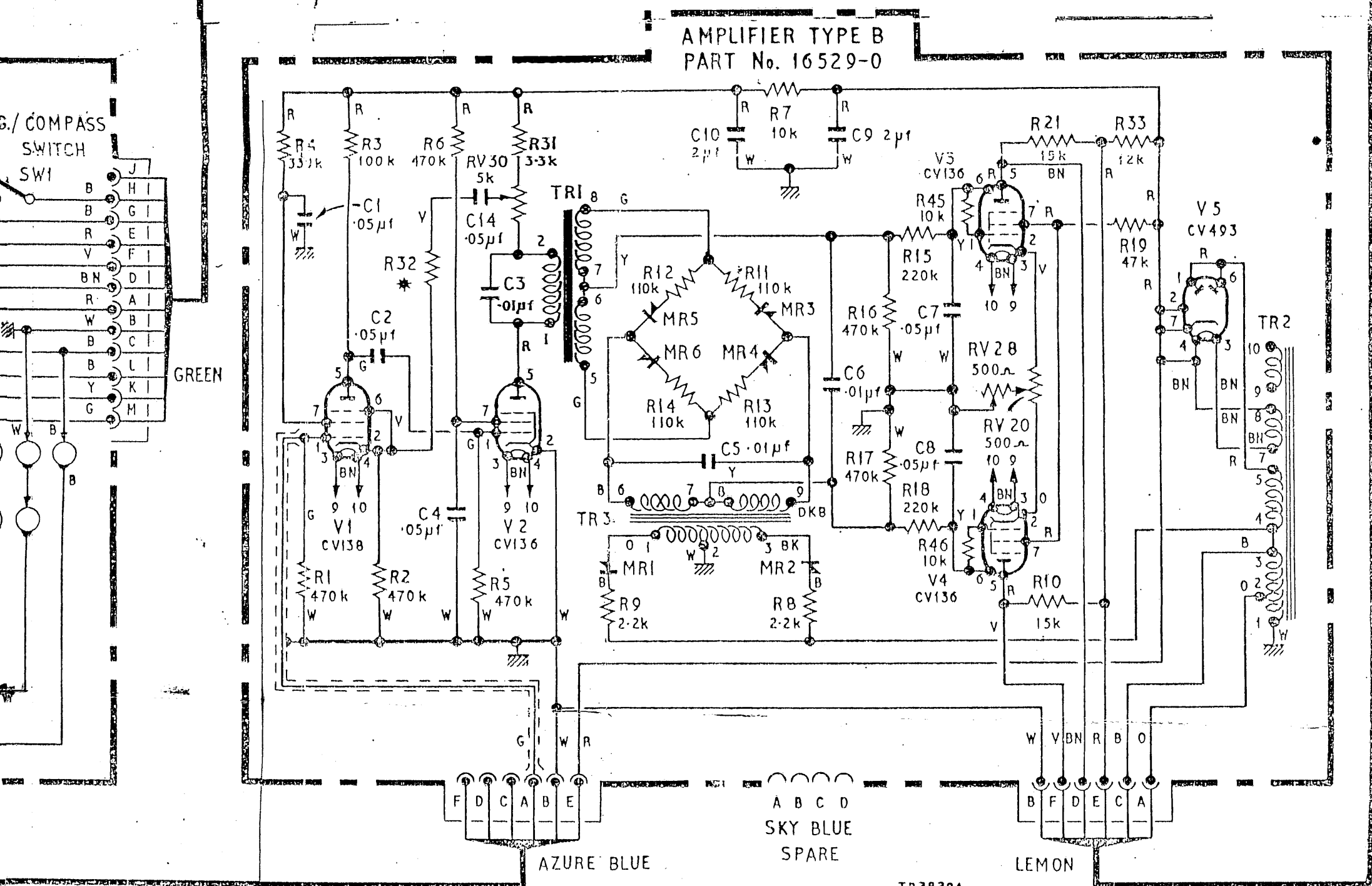
EQUIPMENT CIRCUIT DIAGRAM GYROSYN COMPASS TYPE C.L.I.
