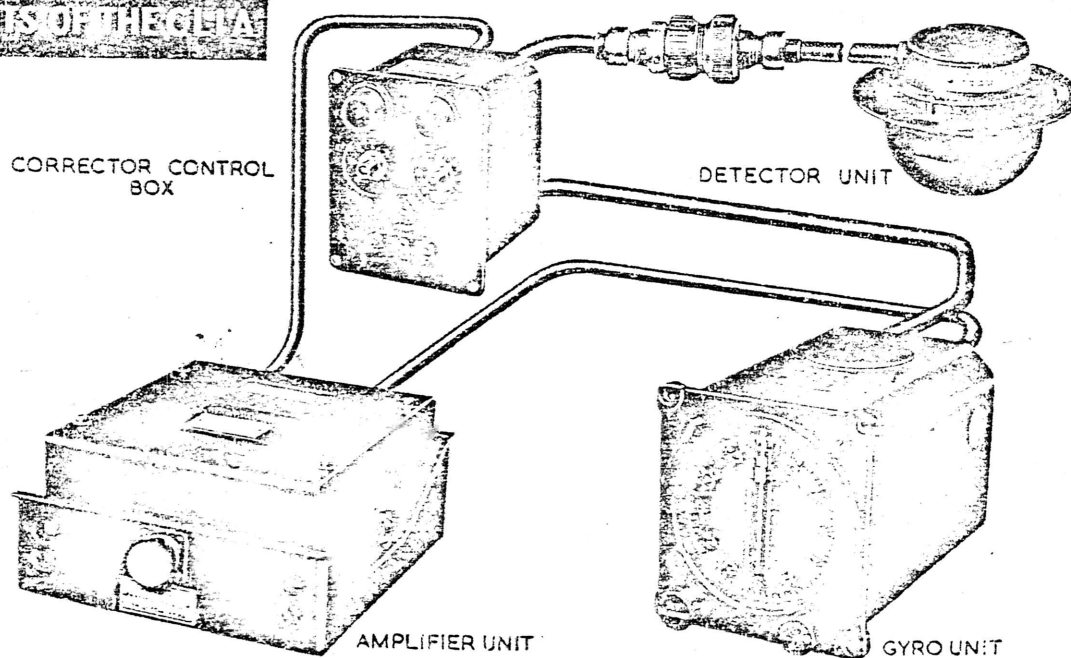
Fig. 1 Units of the C.L.I and C.L.IA Gyrosyn Compass
